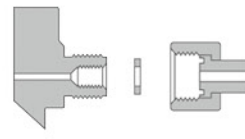
CGA 180 0.625" -18 UNF 2A RH EXT. with Gasket
